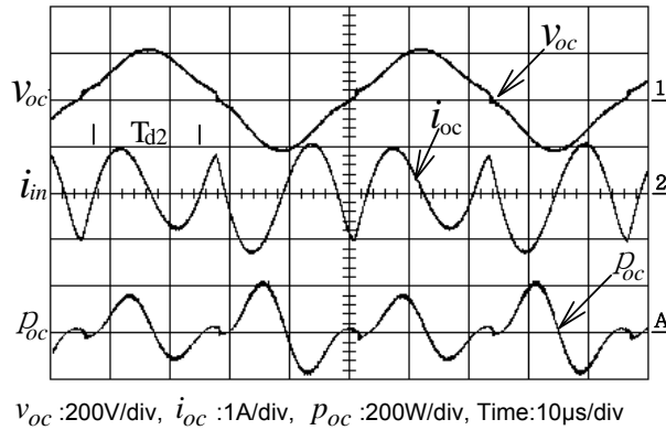
Figure 7. The measured waveforms of the open-circuited test with an external inductor L_r=200\mu\text{H} .
